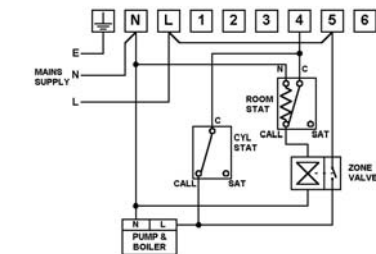
3. Fully Pumped System with RoomStat and two port spring return valve (with auxiliary switch) on Heating circuit
